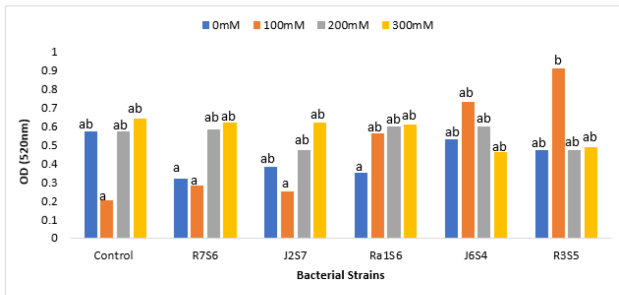
Fig. 17. Effects of 0 mM, 100 mM, 200 mM and 300 mM NaCl conc. on proline content of barley. Color bars show mean of 8 replicates. Different alphabets represent a significant difference in mean values by using Duncan's multiple range test ( P \leq 0.05 ).
