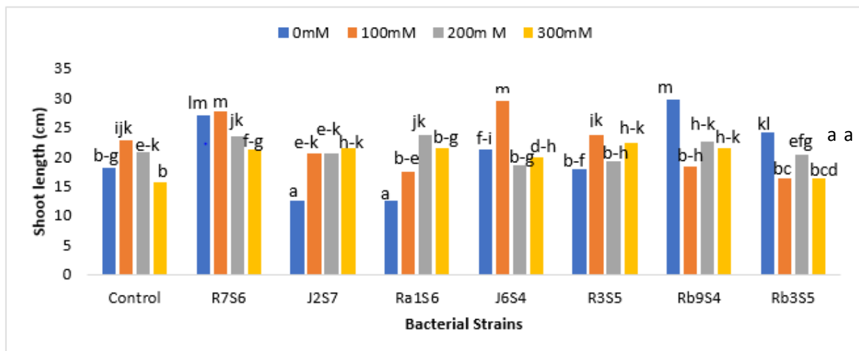
Fig. 7. Effects of Bacillus and Halomonas strains on the shoot length (0-300 mM) of barley grow under laboratory conditions amended with different levels of salinities. Color bars show the different levels of salt stress. Significant difference in mean values was represented by different alphabets using Duncan's multiple range test ( P \leq 0.05 ).
