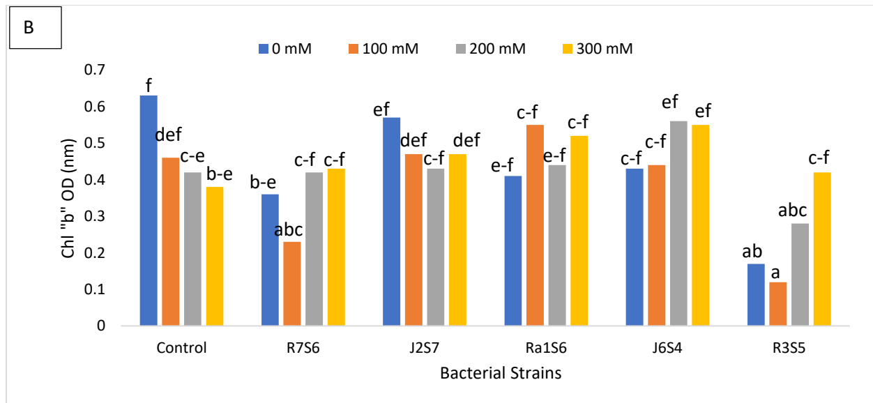
Fig. 15. Effect of different NaCl concentrations (0-300 mM) on chlorophyll content of plants (A) Chl "a" (B) Chl "b". Bars represent mean of 8 replicates. Significant difference in mean values was represented by different alphabets using Duncan's multiple range test ( P \leq 0.05 ).
