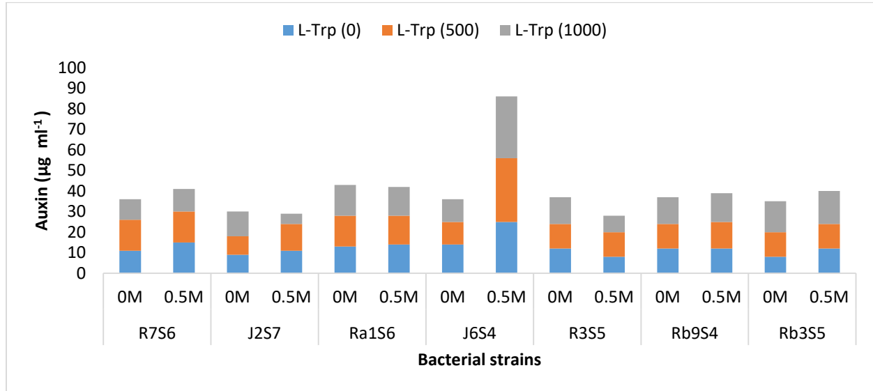
Fig. 1. Effect of different concentrations of NaCl and L-tryptophan on bacterial auxin production. Colored bars represent mean of 4 replicates.
