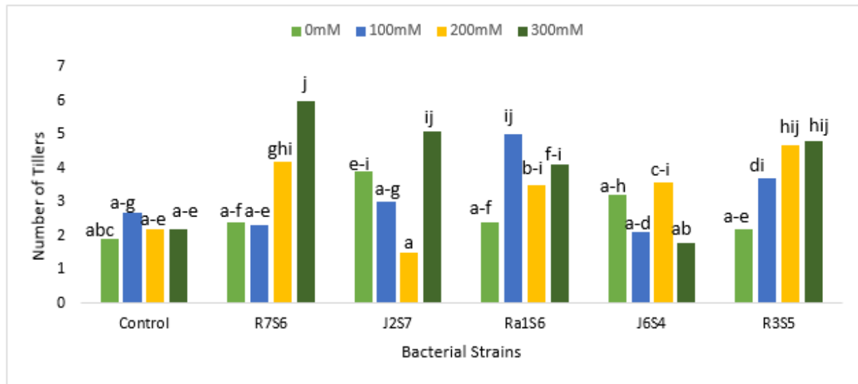
Fig. 14. Effects of Bacillus and Halomonas strains on number of tillers (0-300 mM) of barley grown under natural conditions amended with different levels of salinities. Color bars show the different levels of salt stress. Significant difference in mean values was represented by different alphabets using Duncan's multiple range test ( P \leq 0.05 ).
