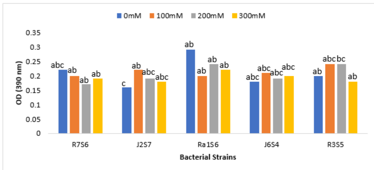
Fig. 16. Effects of 0 mM, 100 mM, 200 mM and 300 mM NaCl conc. on catalase content of barley. Color bars show mean of 8 replicates. Different alphabets represent a significant difference in mean values by using Duncan's multiple range test ( P \leq 0.05 ).
