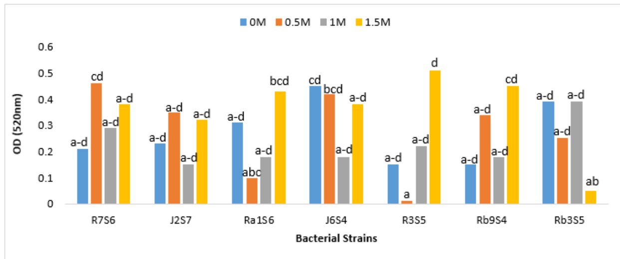
Fig. 4. Proline production at 0 M, 0.5 M, 1 M and 1.5 M NaCl. Each bar represents mean of 4 replicates. Significant difference in mean values was represented by different alphabets using Duncan's multiple range test ( P \leq 0.05 ).
