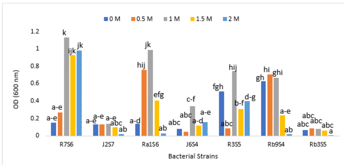
Fig. 3. Effects of increasing NaCl stress (0-2M) on bacterial growth. Colored bars showed the bacterial growth at different NaCl stress.
