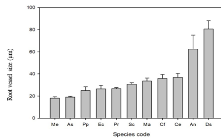
Fig. 3. Root vessel size across species studied. Species codes are listed in Table 1
