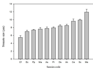
Fig. 5: Stomata size across species studied. Species codes are listed in Table 1.
