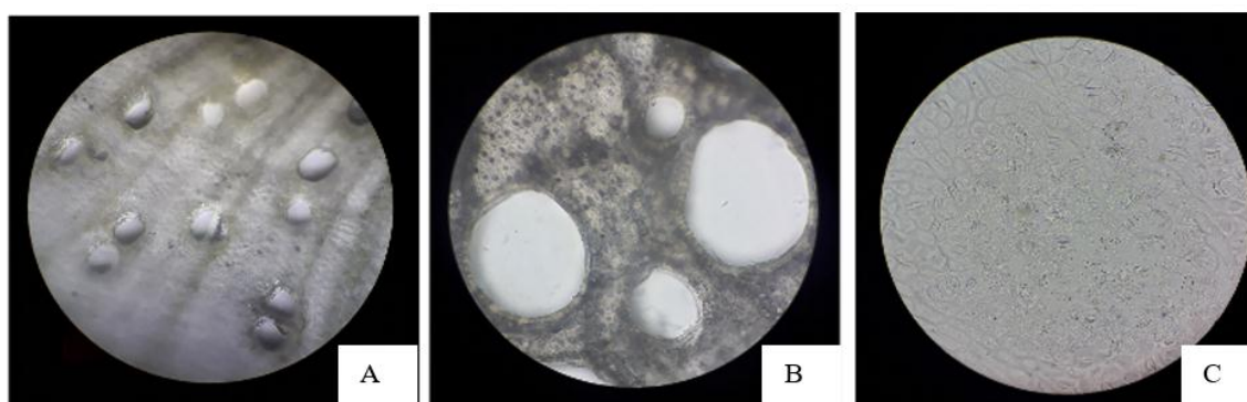
Plate 5: Dalbergia sissoo , A (Stem xylem vessels), B (Root xylem vessels), C (stomata)
